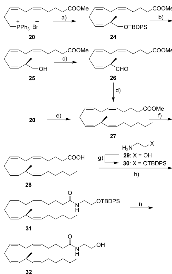
Scheme 5. Synthesis of 32 . Reagents and conditions: a) KHMDS, THF, –78––60°C, 20 min, then 3 , –115–0°C, 3 h, 61 %; b) TBAF, THF, 0°C to RT, 1.5 h, 85 %; c) Dess–Martin periodinane, 0°C to RT, 75 min; d) \text{CH}_3(\text{CH}_2)_5\text{P}^+\text{Ph}_3\text{Br}^- , KHMDS, THF, 0°C, 40 min, then addition of 26 , –115––100°C, 50 min, 65 % from alcohol 25 ; e) KHMDS, THF, –78––60°C, 20 min, then 11 , –98–0°C, 2.5 h, 22 %; f) LiOH, THF/ \text{H}_2\text{O} , RT, 24 h, 86 %; g) TBDPSCl, imidazole, \text{CH}_3\text{CN} , 0°C, 30 min, 97 %; h) carbonyldiimidazole, THF, RT, 2 h, then 30 , RT, 1 h, 91 %; i) TBAF, THF, 0°C to RT, 1 h, 88 %.
