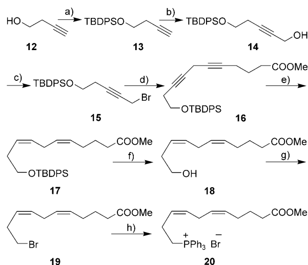
Scheme 3. Synthesis of alkenyl phosphonium salt 20 . Reagents and conditions: a) TBDPSCl, imidazole, THF, 0^\circ\text{C} , 1.5 h, 99%; b) n BuLi, THF, 0^\circ\text{C} , 1.5 h, then (\text{CH}_2\text{O})_n , -50^\circ\text{C} to RT, 1.5 h, 73%; c) \text{CBr}_4 , \text{Ph}_3\text{P} , \text{CH}_2\text{Cl}_2 , 0^\circ\text{C} to RT, 3 h, 85%; d) \text{CH}\equiv\text{C}-(\text{CH}_2)_3-\text{COOMe} , \text{Cs}_2\text{CO}_3 , NaI, CuI, DMF, RT, 2.5 h, 95%; e) \text{Ni}(\text{OAc})_2 , \text{NaBH}_4 , ethylenediamine, \text{H}_2 , MeOH, RT, 2 h, 85%; f) TBAF, THF, 0^\circ\text{C} to RT, 1.5 h, 93%; g) \text{CBr}_4 , \text{Ph}_3\text{P} , \text{CH}_2\text{Cl}_2 , -25 – 0^\circ\text{C} , 1.5 h, 96%; h) \text{Ph}_3\text{P} , \text{CH}_3\text{CN} , 72 – 75^\circ\text{C} , 8 days, 95%. TBAF=tetrabutylammonium fluoride.
