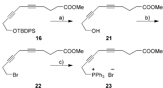
Scheme 4. Synthesis of alkynyl phosphonium salt 23 . Reagents and conditions: a) TBAF, THF, 0°C, 2 h, 84 %; b) \text{CBr}_4 , \text{Ph}_3\text{P} , \text{CH}_2\text{Cl}_2 , –16°C, 2 h, 98 %; c) \text{Ph}_3\text{P} , \text{CH}_3\text{CN} , 70–72°C, 7 days, 88 %.
