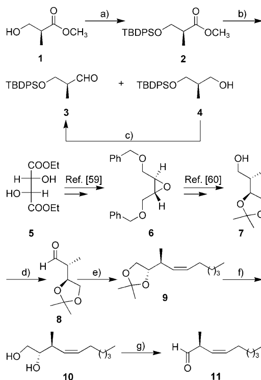
Scheme 2. Synthesis of chiral aldehydes 3 and 11 . Reagents and conditions: a) TBDPSCl, imidazole, \text{CH}_2\text{Cl}_2 , 0^\circ\text{C} to RT, 1.5 h, 98%; b) DIBAL-H, \text{CH}_2\text{Cl}_2 , -110 – -90^\circ\text{C} , 20 min, 61% for 3 and 37% for 4 ; c) Dess–Martin periodinane, 0^\circ\text{C} to RT, 45 min, 90%; d) PCC, \text{CH}_2\text{Cl}_2 , 4 Å molecular sieves, RT, 2.5 h, 93%; e) \text{CH}_3(\text{CH}_2)_5\text{P}^+\text{Ph}_3\text{Br}^- , KHMDS, THF, 10^\circ\text{C} , 50 min, then 8 , -98^\circ\text{C} , 1 h, 50%; f) \text{BF}_3\cdot\text{CH}_3\text{COOH} , MeOH, 0^\circ\text{C} , 1 h, 84%; g) \text{Pb}(\text{OAc})_4 , \text{CH}_2\text{Cl}_2 , -78^\circ\text{C} , 1.5 h, 97%. PCC=pyridinium chlorochromate, KHMDS=potassium bis(trimethylsilyl)amide.
