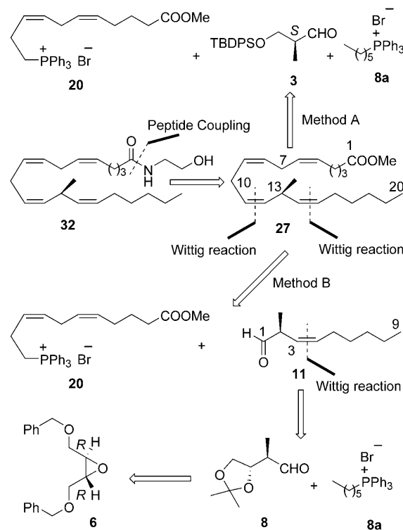
Scheme 1. Retrosynthetic analysis of (13 S )-methylanandamide 32 . TBDPS = tert -butyldiphenylsilyl.
