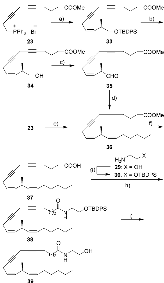
Scheme 6. Synthesis of the conformationally partially extended (13 S )-methyl analogue 39 . Reagents and conditions: a) KHMDS, THF, -78^{\circ}\text{C} , 50 min, then 3 , -98 – 0^{\circ}\text{C} , 2.5 h, 58 %; b) TBAF, \text{CH}_3\text{COOH} , THF, 0^{\circ}\text{C} to RT, 20 h, 76 %; c) Dess–Martin periodinane, 0^{\circ}\text{C} , 2 h; d) \text{CH}_3(\text{CH}_2)_3\text{P}^+\text{Ph}_3\text{Br}^- , KHMDS, THF, 10^{\circ}\text{C} , 40 min, then addition of 35 , -98^{\circ}\text{C} , 1 h, 58 % from alcohol 34 ; e) KHMDS, THF, -78^{\circ}\text{C} , 50 min, then 11 , -98 – 0^{\circ}\text{C} , 2.5 h, 21 %; f) LiOH, THF/ \text{H}_2\text{O} , RT, 7 h, 82 %; g) TBDPSCI, imidazole, \text{CH}_3\text{CN} , 0^{\circ}\text{C} , 30 min, 91 %; h) Carbonyldiimidazole, THF, RT, 2 h, then 30 , RT, 1 h, 97 %; i) TBAF, \text{CH}_3\text{COOH} , THF, 0^{\circ}\text{C} to RT, 20 h, 75 %.
